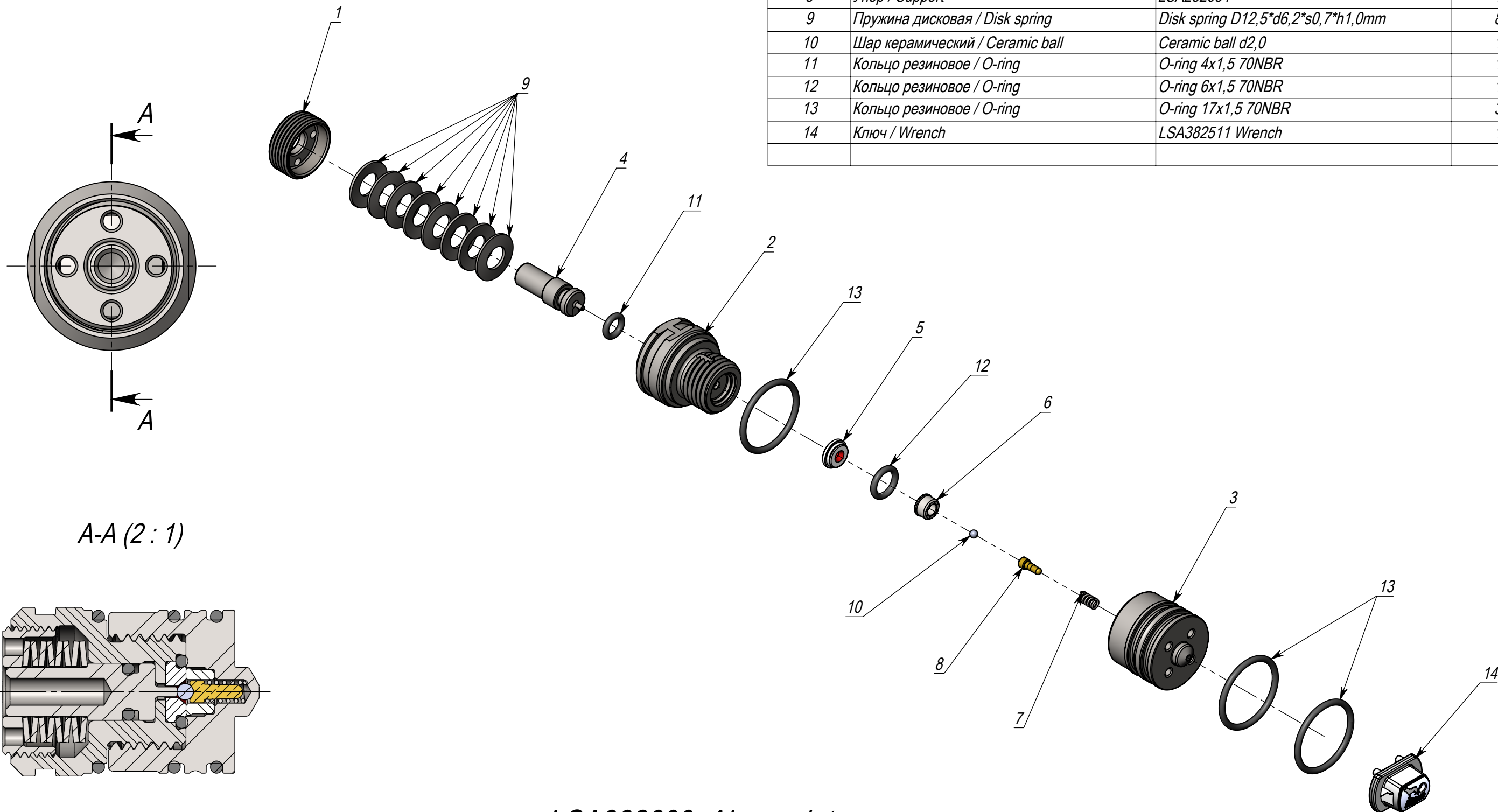
LSA382600 Air regulator
